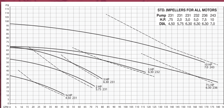
Pump Performance Curves
