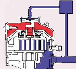
Unloaded Scroll separated no compression
