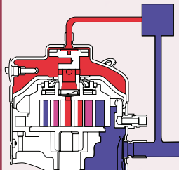
Loaded Scroll engaged full compression
