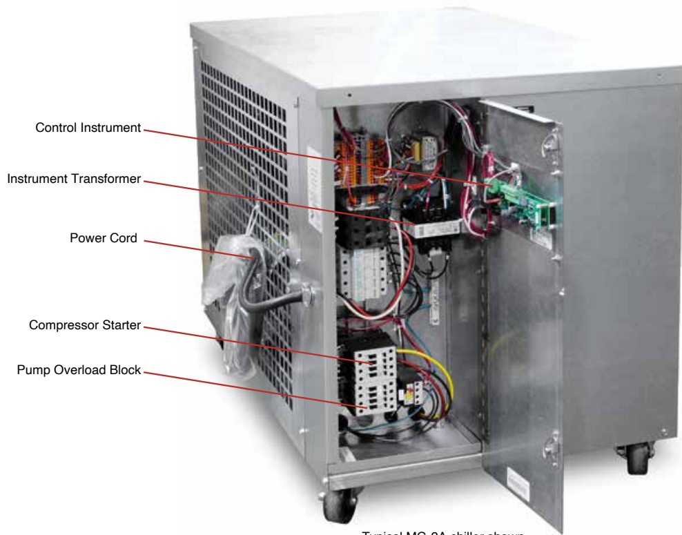
Typical MG-2A chiller shown
