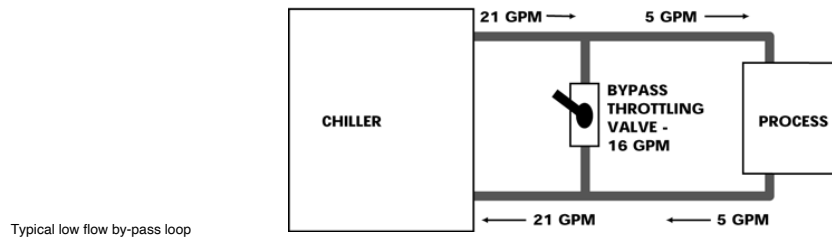
Typical low flow by-pass loop
