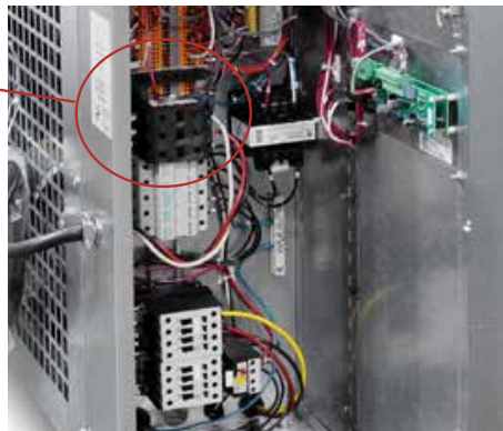
Power Entry Terminal Block shown on a typical MG-2A chiller.
